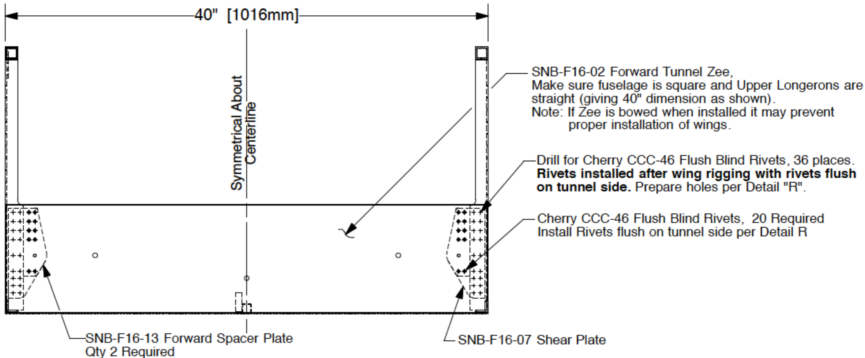
View K-K View Looking forward at Forward Tunnel Zee Scale: 1/8
