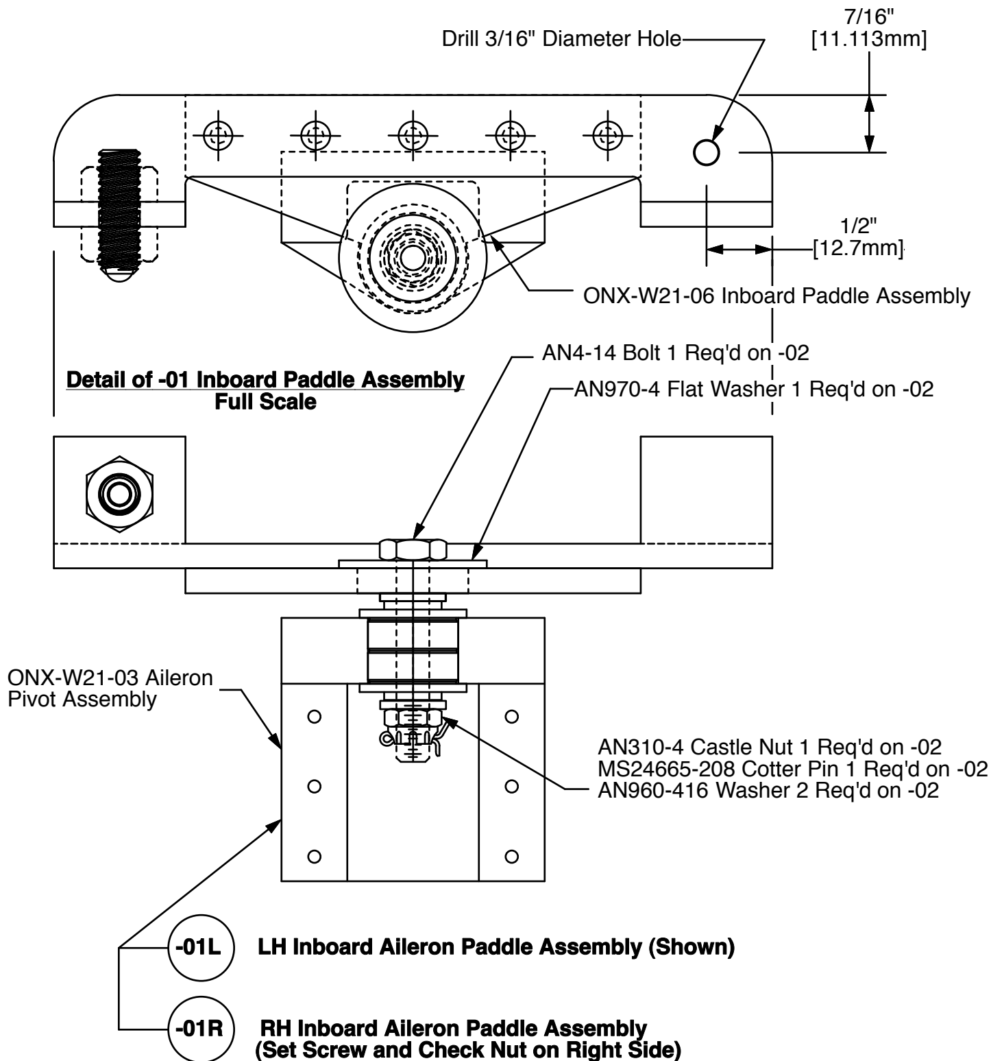
Inboard Aileron Control Push Road attach hole detail for ONX-W21-01R/-01L Inboard Aileron Paddle Assembly.
