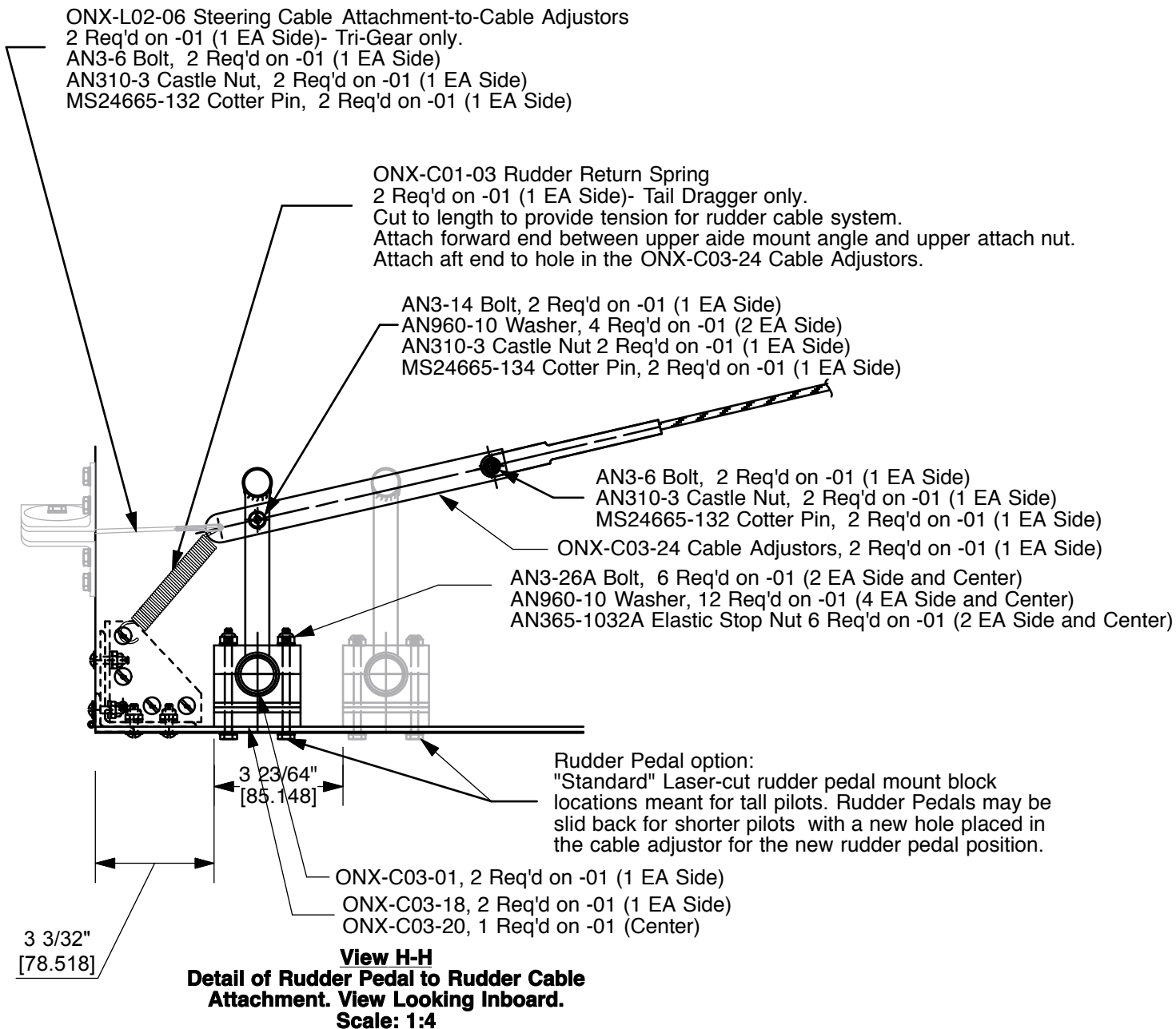
ONX-C01 Rev E View H-H- Showing Tri-Gear Steering Cable Attachment at Rudder Pedal
