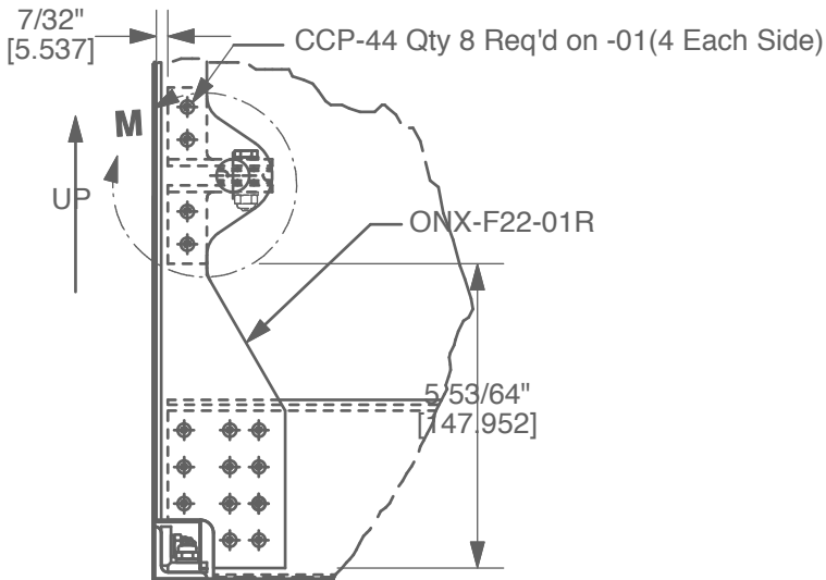
View K-K Aft Pulley Installation at #1 Former Position Scale 1:4
