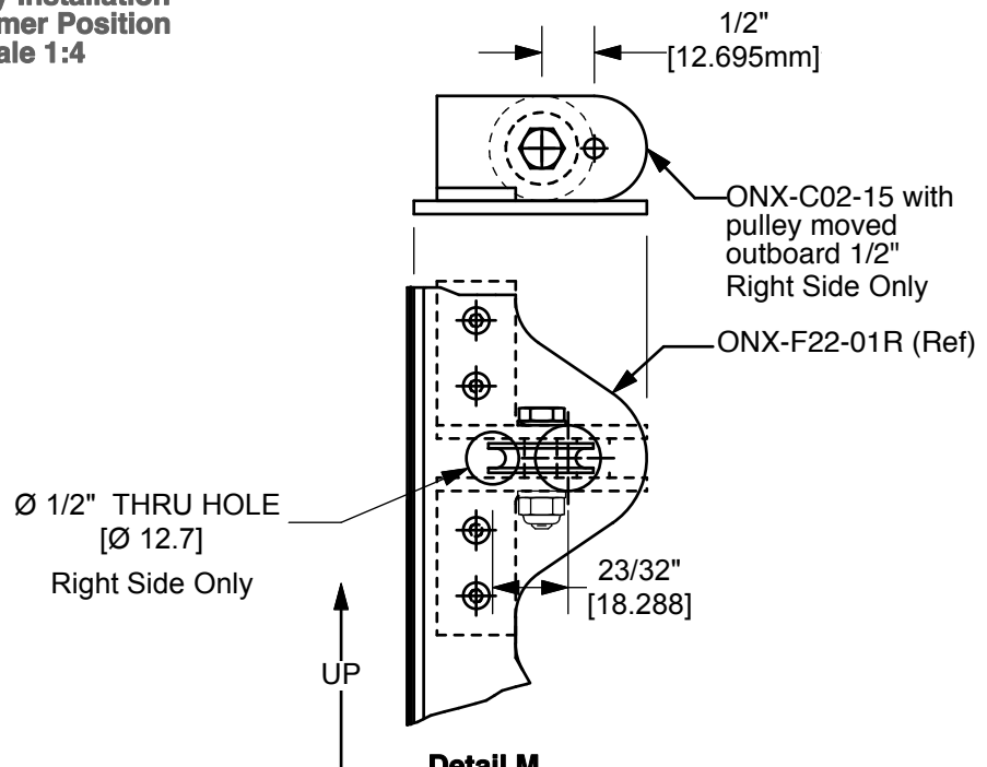
Detail M Modification of ONX-C02-15 Rudder Cable Pulley Bracket for Right Side Scale: 1/2
