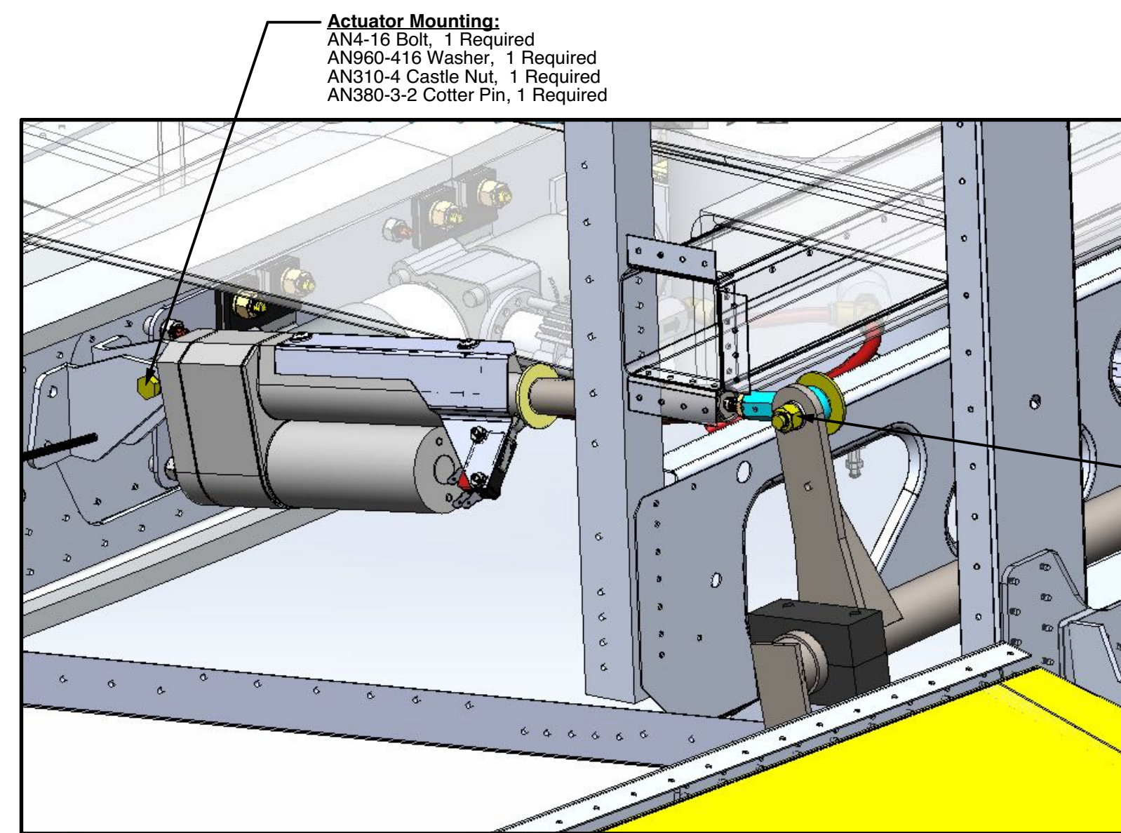
Detail C Flap Actuator and Rod Assembly Installation
