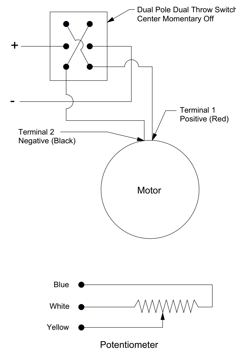
Detail F Flap Actuator Wiring Schematic
