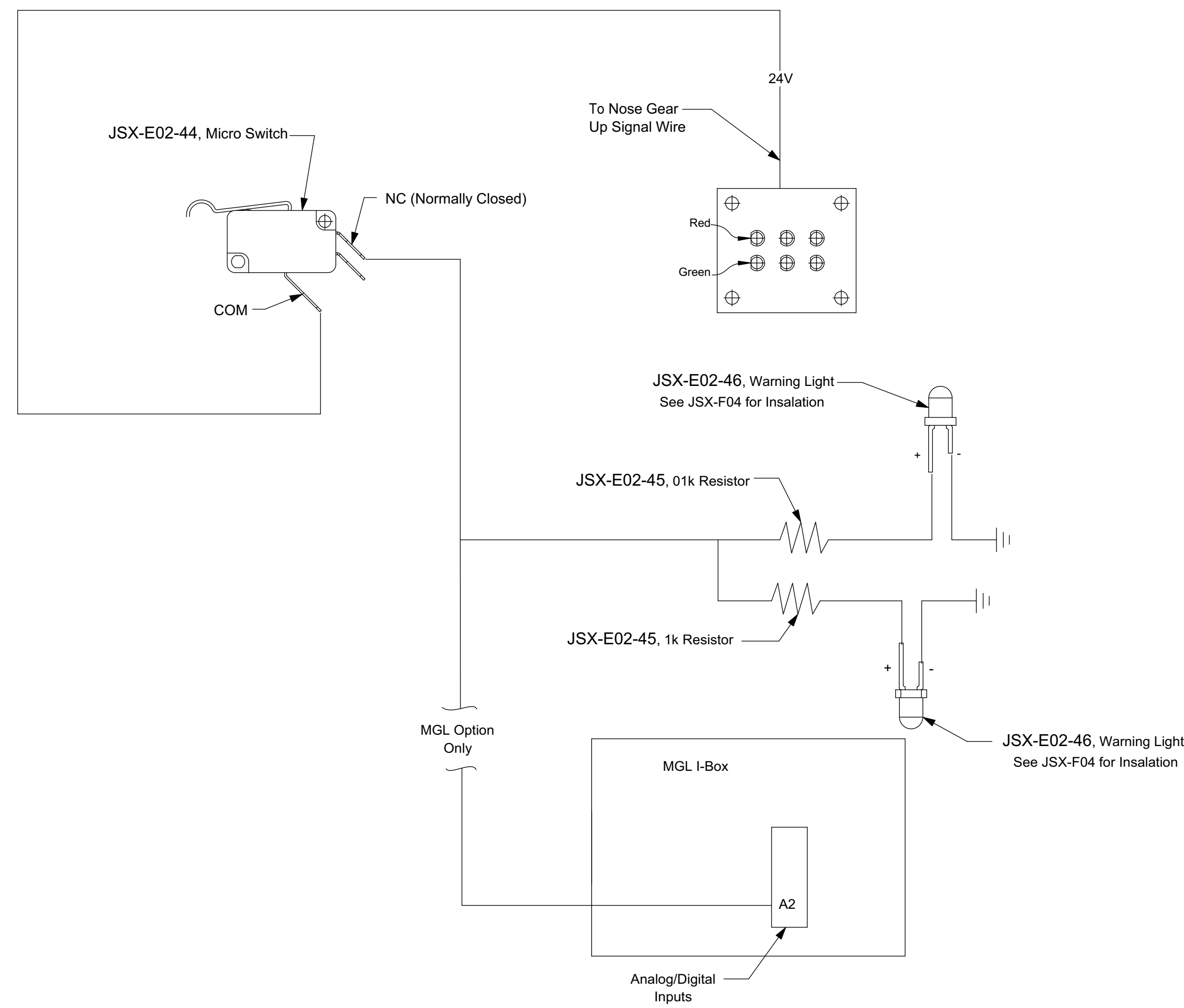
Detail E Warning Lights Wire Diagram
