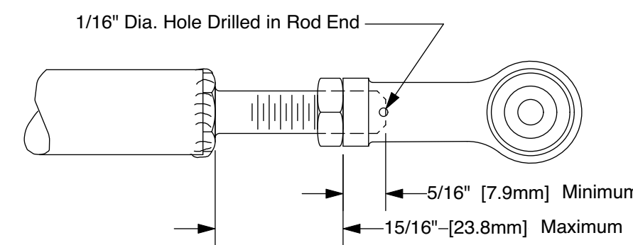
Detail D Minimum Thread Engagement for Rod End Control Pushrod Threads MUST Extend to Witness Hole for Proper Installation
