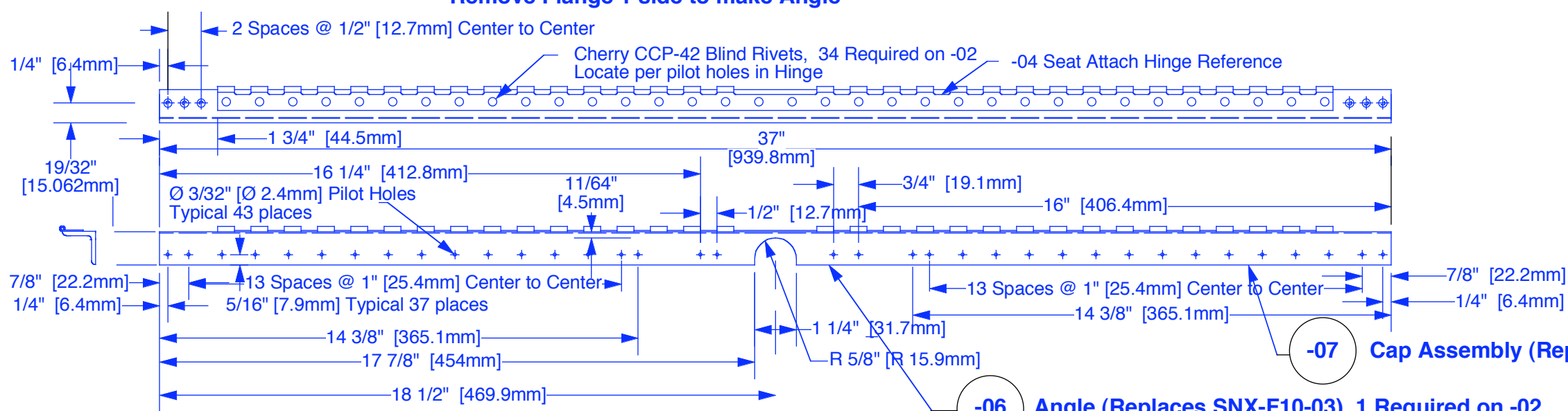
-05 Angle (Refer to SNX-F10-01 for all dimensions not given on this view) Make from SNX-Z04-03 3 1/2\" Channel Stock Remove Flange 1 side to make Angle
