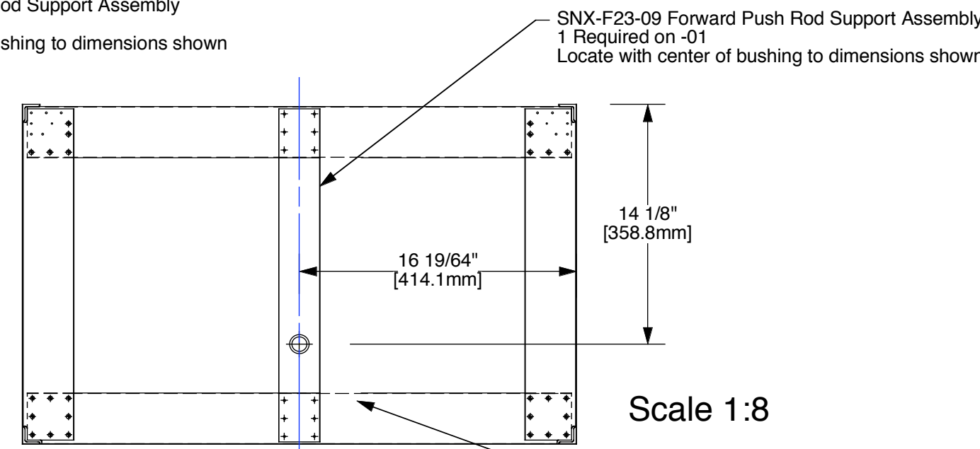
Section P-P View Looking Aft at Push Rod Support
