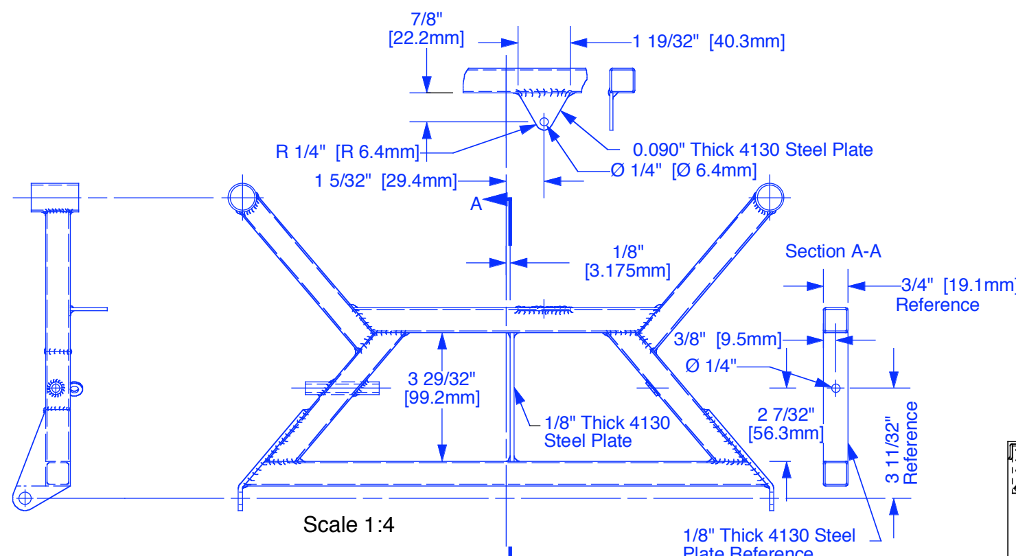
SNX-C05-08 Control Stick Frame Assembly for Lowered Seat 1 Required on -01, Weld Frame Assembly together using number 7 welding rod
