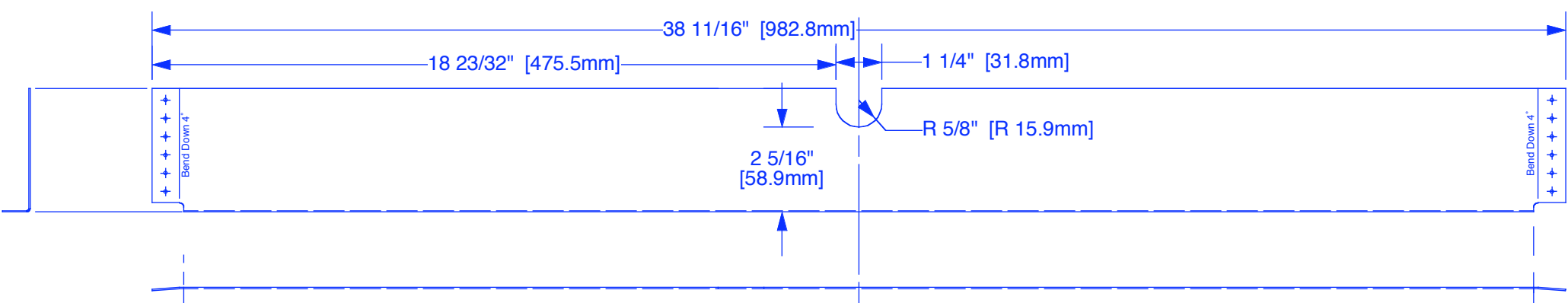
-05 Angle (Refer to SNX-F10-01 for all dimensions not given on this view) Make from SNX-Z04-03 3 1/2\" Channel Stock Remove Flange 1 side to make Angle
