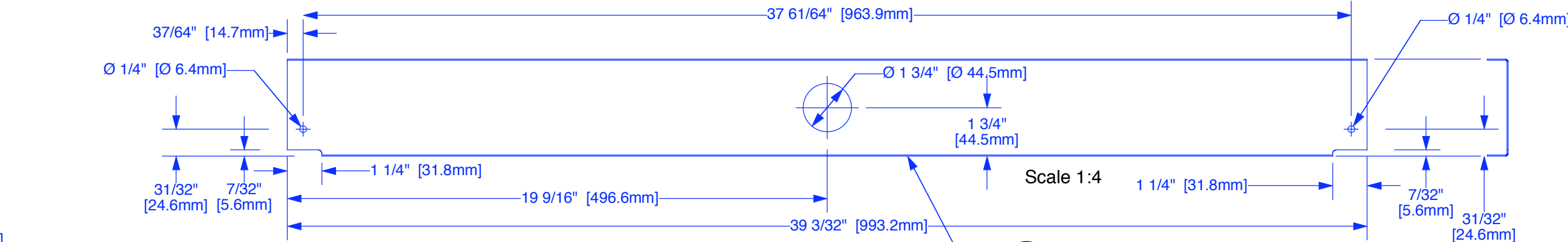
(Replaces SNX-F03-02 Channel) Channel, 1 Required on -01 Make from SNX-Z04-03 3 1/2\" Channel Stock (40\" [1016mm] long)
