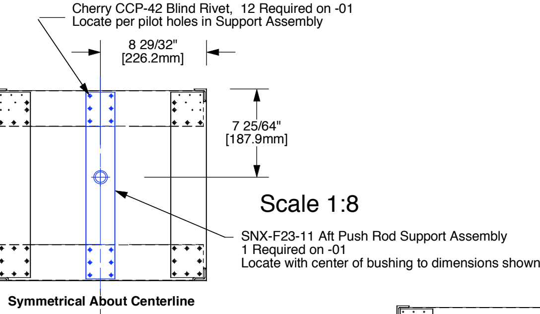
Section N-N View Looking Aft at Push Rod Support
