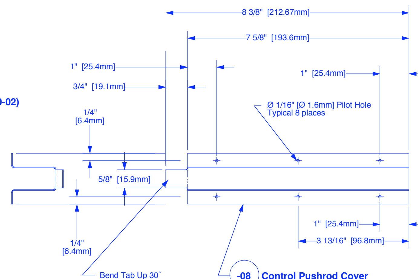
-08 Control Pushrod Cover 1 Required on -01 Make from XNS-Z04-01 Hat (Hat Section Available for Purchase from Sonex)
