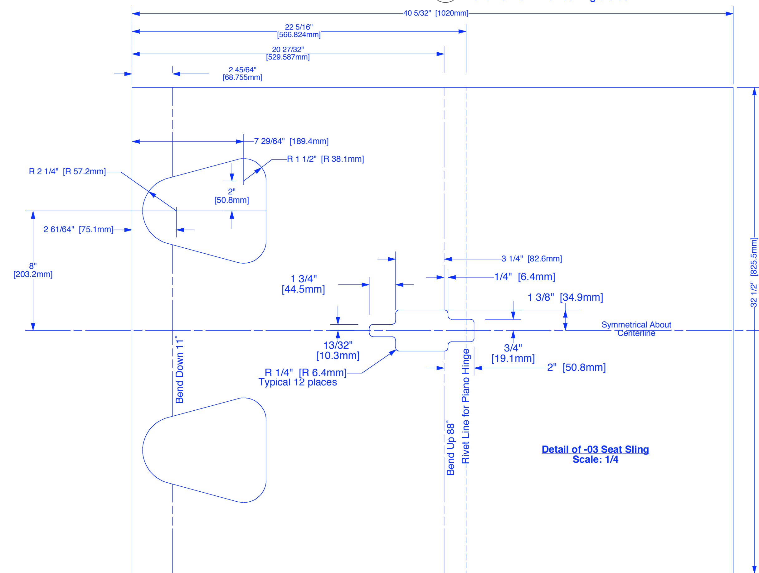
-03 Dropped Seat Sling, 1 Required on -01 .025\" Thick 6061-T6 Aluminum Sheet 1/16\" [1.6mm] Bend Radius
