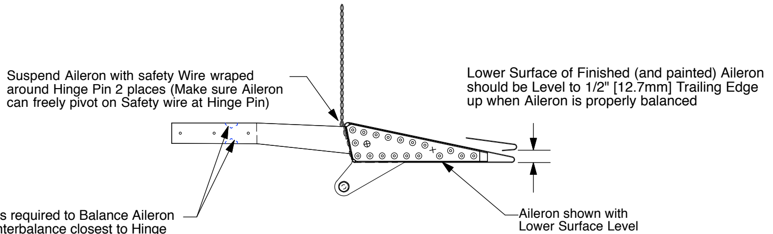
Detail of Aileron Balancing Scale: 1/4
