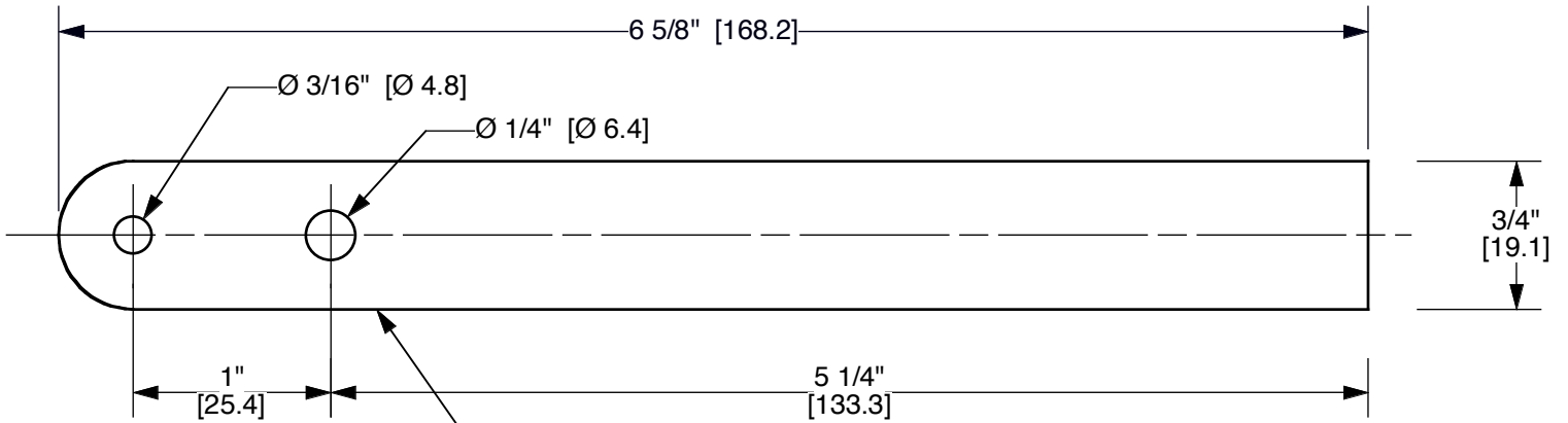
-03L Cable Adjuster Scale: Full Make from .190" thick 6061-T6 Aluminum
